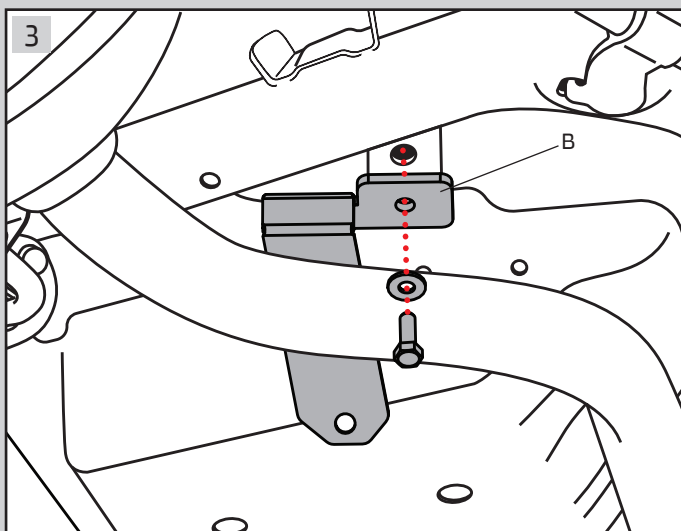
Connect front bracket (B) using original M8 (8.8) bolt Tightening torque 40Nm
