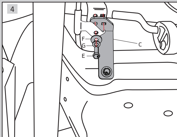
Connect front bracket (C) using kit M8 (8.8) bolt Tightening torque 21Nm
