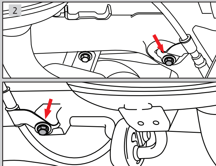
Open 2 bolts. Save the bolts for later use.
