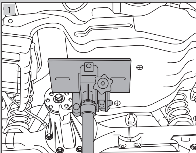
Support the fuel tank with Jack
