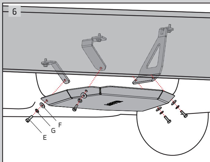
Connect the fuel tank skid plate Using kit M8 (8.8) bolts Tightening torque 25Nm
