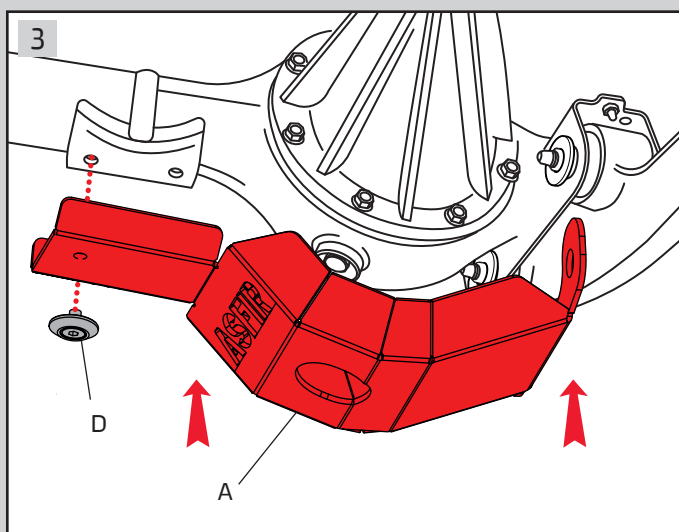
Connect differential skid plate (A) to bracket (B 1 ) using kit bolt (D) Tightening torque M8(8.8)-25Nm
