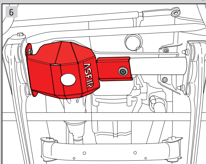
Tightening torque M12 (8.8)-90Nm, M8 (8.8)-25Nm
