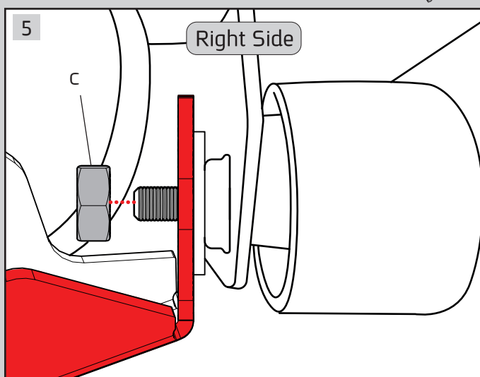
Using kit nut (C) Add thread locker glue to original connection
